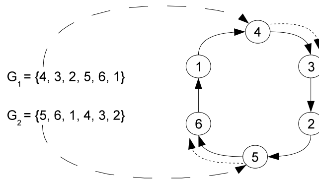
Figure 4. Two different chromosomes ( G_1, G_2 ) coding the same route 4 \rightarrow 3 \rightarrow 2 \rightarrow 5 \rightarrow 6 \rightarrow 1 .
